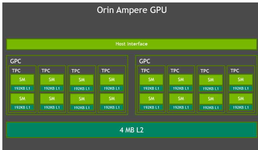
Figure 4: Orin Ampere GPU Block Diagram
