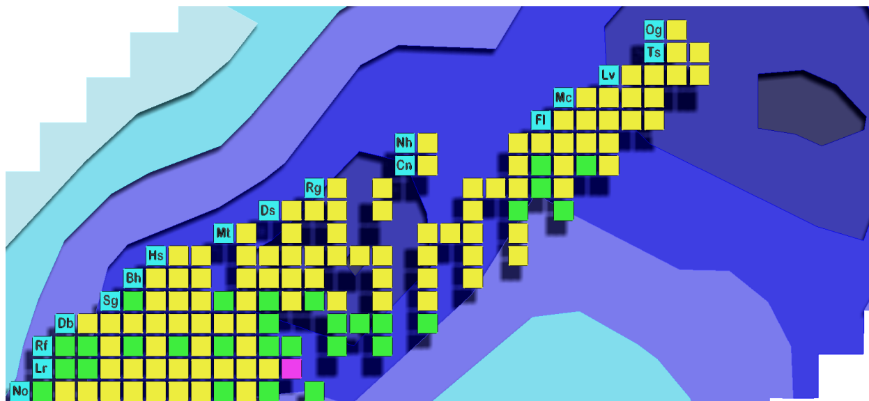
Figure 1.1: Nuclear Chart with the Island of Stability. Known isotopes are shown by their preferred decay mode, either alpha (yellow), beta (magenta) or spontaneous fission (green). These are on a backdrop of predicted shell effects from [Sob01].
