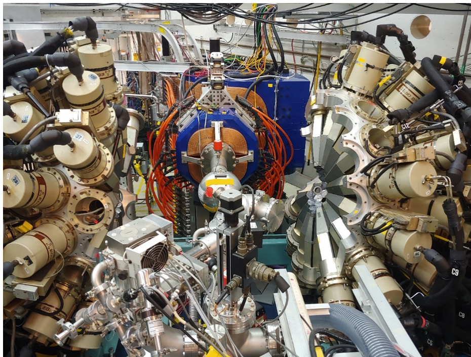
Figure 3.1: Looking downstream along the beamline into AGFA at ANL. Gammashpere is open in this image, but closes around the spherical target chamber, providing a sensitive setup for prompt \gamma -ray spectroscopy of transfermium isotopes. Figure taken from https://www.anl.gov/phy/argonne-gasfilled-analyzer .
